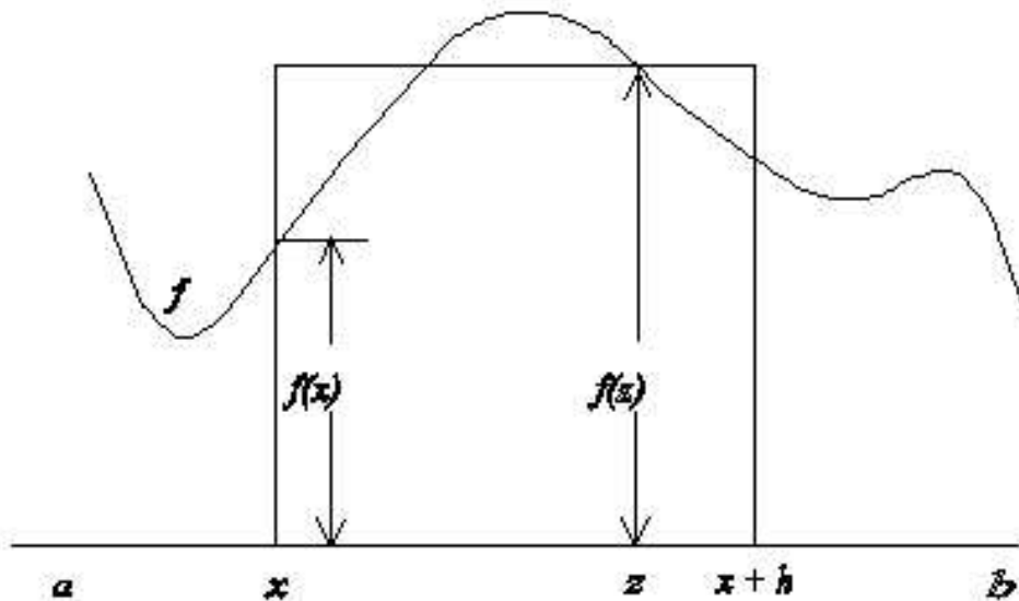
Figure 5-1. Geometric setup of the proof of the First Fundamental Theorem.
